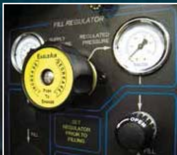
Exclusive regulator design that prevents unintentional adjustment in compliance with NFPA 1901 standards
